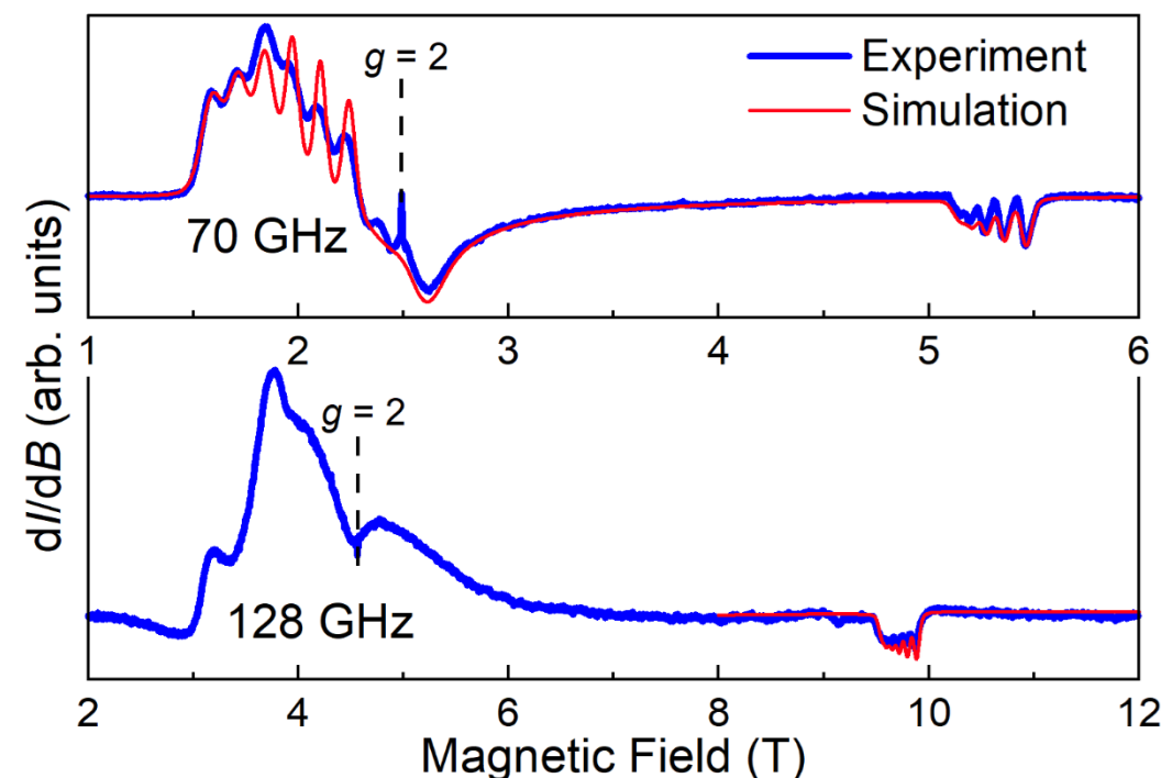
Fig. 1. Multi-frequency, high-field EPR spectra of the [\text{K}(\text{crypt})]^+[\text{Cp}_3\text{Pr}^{\text{II}}]^- complex, which has an effective spin- 1/2 ground state. Different components of the Landé g -tensor are well-resolved at the highest frequency. Spectral simulations then allow determination of the g - and A -tensor components.
