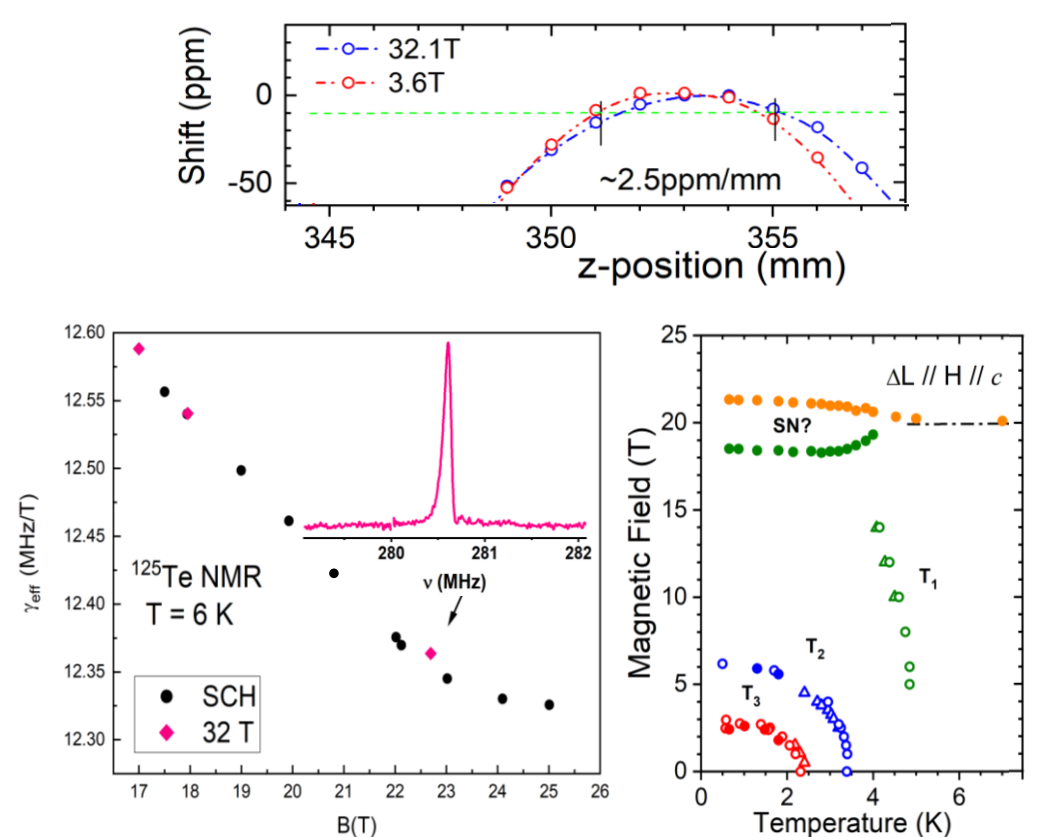
Figure: (Top) Magnet field profile of the new magnet along the z-axis at 32.1T and 3.6T measured with 63 Cu NMR. (Left) 125 Te spectral line and effective gamma with respect to magnetic field. Black circles are from the 36T Series Connected Hybrid while the pink diamonds are from the new HTS 32T magnet. (Right) Phase diagram for H//c highlighting the possible spin-nematic state. [PRB 94 064403 2016] Solid circles are from magnetostriction. Open circles from magnetostriction and thermal expansion. Open triangles from magnetization.
