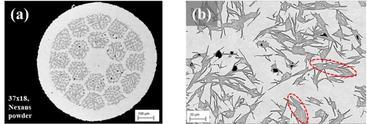
Fig: (a) A cross section view of a Bi-2212 superconducting round wire used in the study, showing 18 bundles, each of which contains 37 superconducting filaments, and (b) a closeup of some of the bundles from the same cross section. The red ovals highlight unwanted filament interconnections that increase magnetization losses. (c) Magnetization loss per cycle as a function of twist length ( L_p ) normalized to wire volume. Losses are very close to - and even below - the ITER specification (red dashed line) for maximum magnetization losses.
